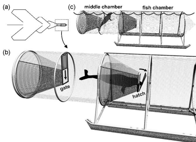
Fig. 1. (a) A trap-net is equipped with a leader, wings and chambers. In a pontoon trap the chambers are made of strong double-layer netting held under tension by rigid hoops; (b) the principle of the capture unit: the non-return gate system installed in the entrance of the middle chamber allows the seal to swim into the middle chamber and towards the entrance of the fish chamber where it pushes the hatch and thereby releases the gate that falls down behind the seal. Attached in the hatch is a release wire that triggers the gate (wire not shown); and (c) the seal is trapped in the chamber where it is still able to reach the surface for air.
